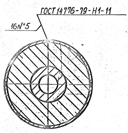
3-3 (1:4)
