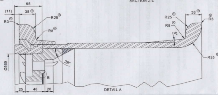
SECTION Z-Z
