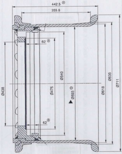
SECTION Z-Z
