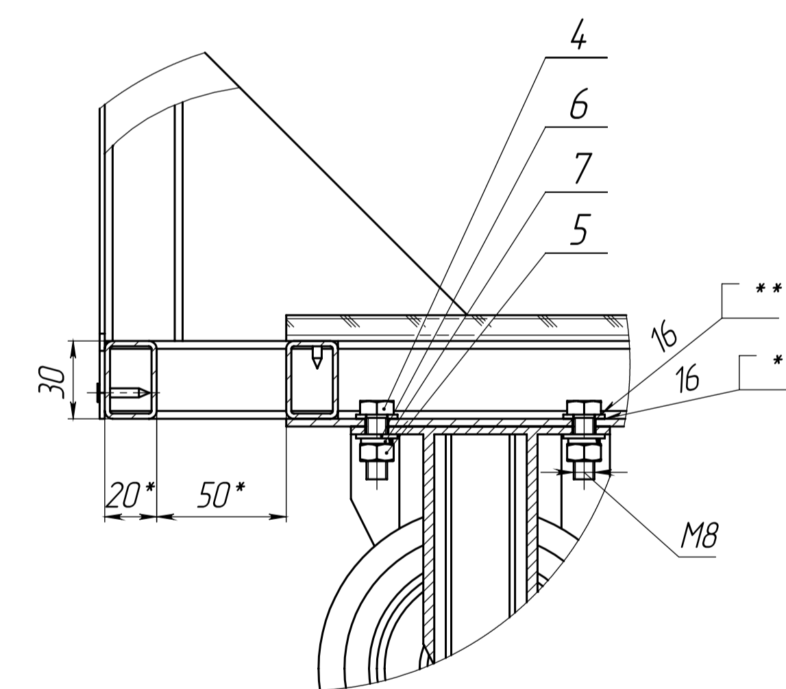
B (1:2)
