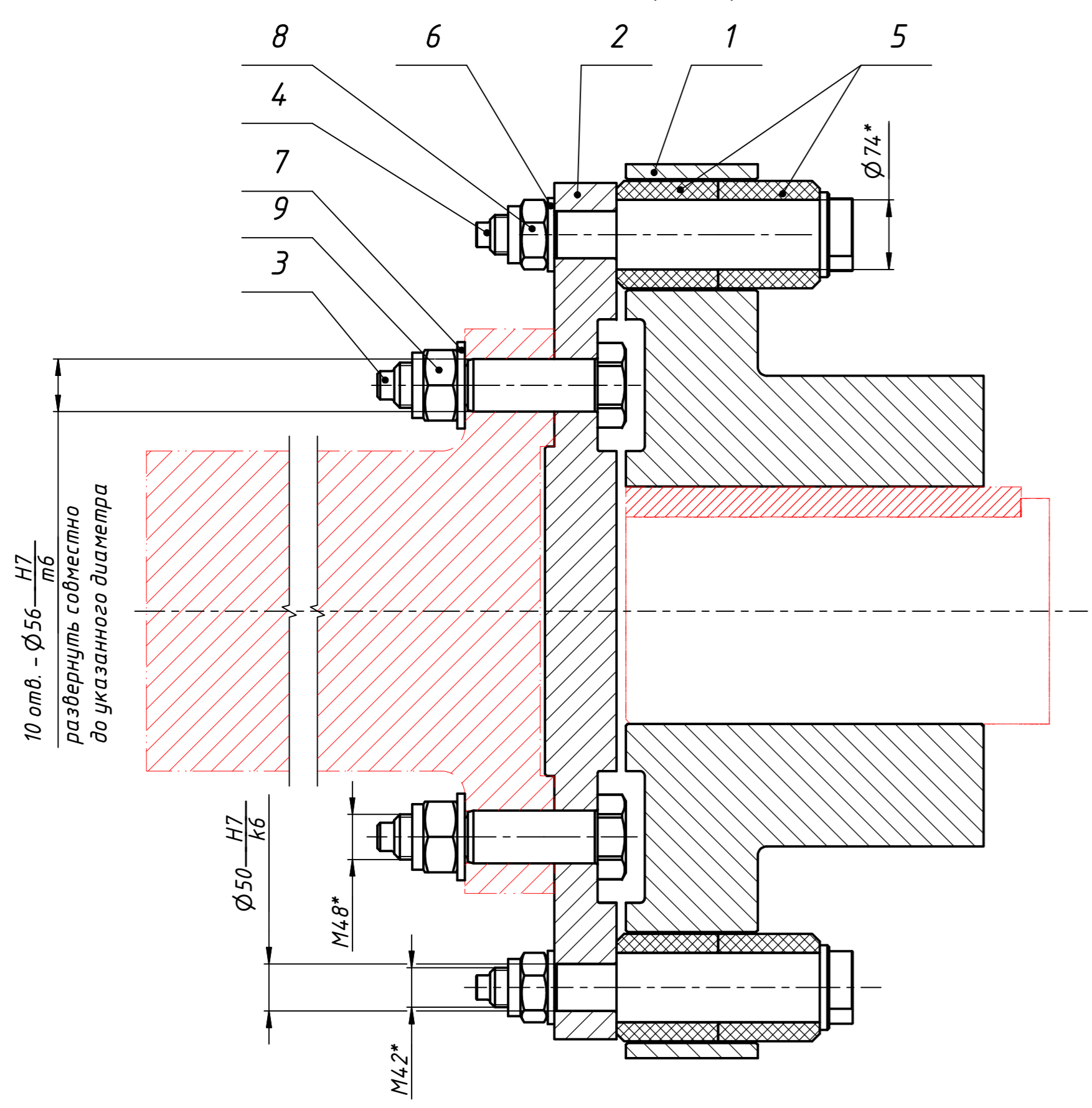
B-B (1:5)
