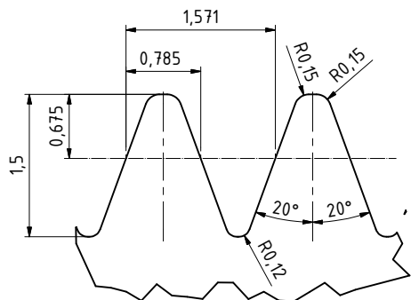
NORMAL TOOTH PROFILE VIEW GOST 10331-81 B ( 20 : 1 )
