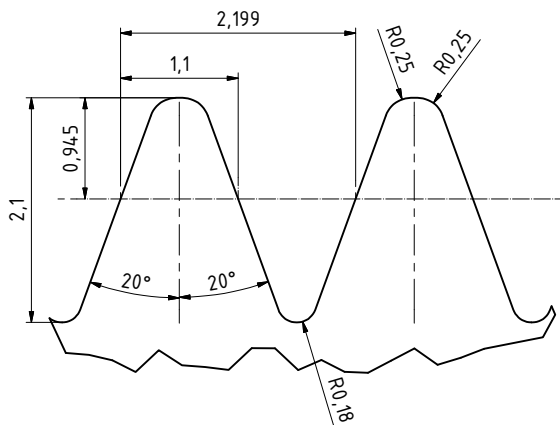
NORMAL TOOTH PROFILE VIEW GOST 10331-81 B ( 20 : 1 )
