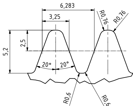
NORMAL TOOTH PROFILE VIEW GOST 9324-80 B ( 5 : 1 )
