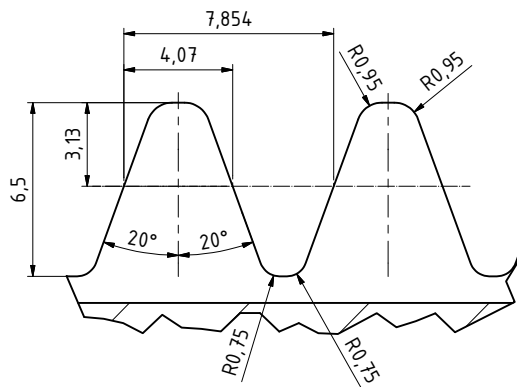
NORMAL TOOTH PROFILE VIEW GOST 9324-80 B ( 5 : 1 )
