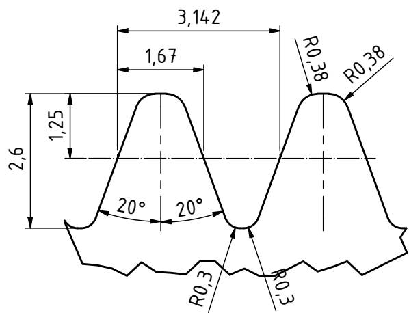
NORMAL TOOTH PROFILE VIEW GOST 9324-80 B ( 10 : 1 )
