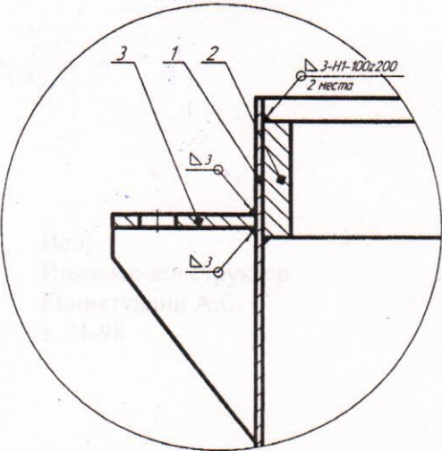
A(1:1)
