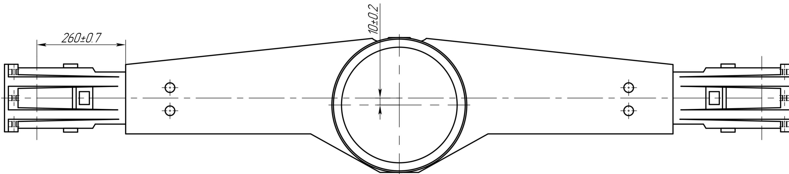
A - A (1:2)
