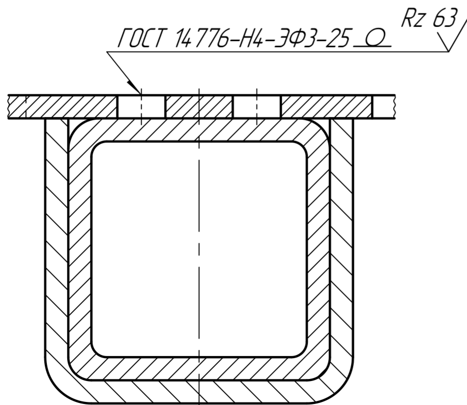
A - A (1:2)
