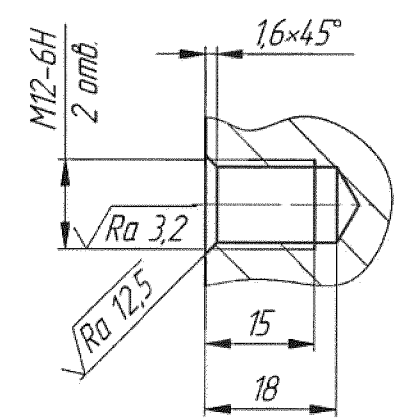
B-B (1:1)
