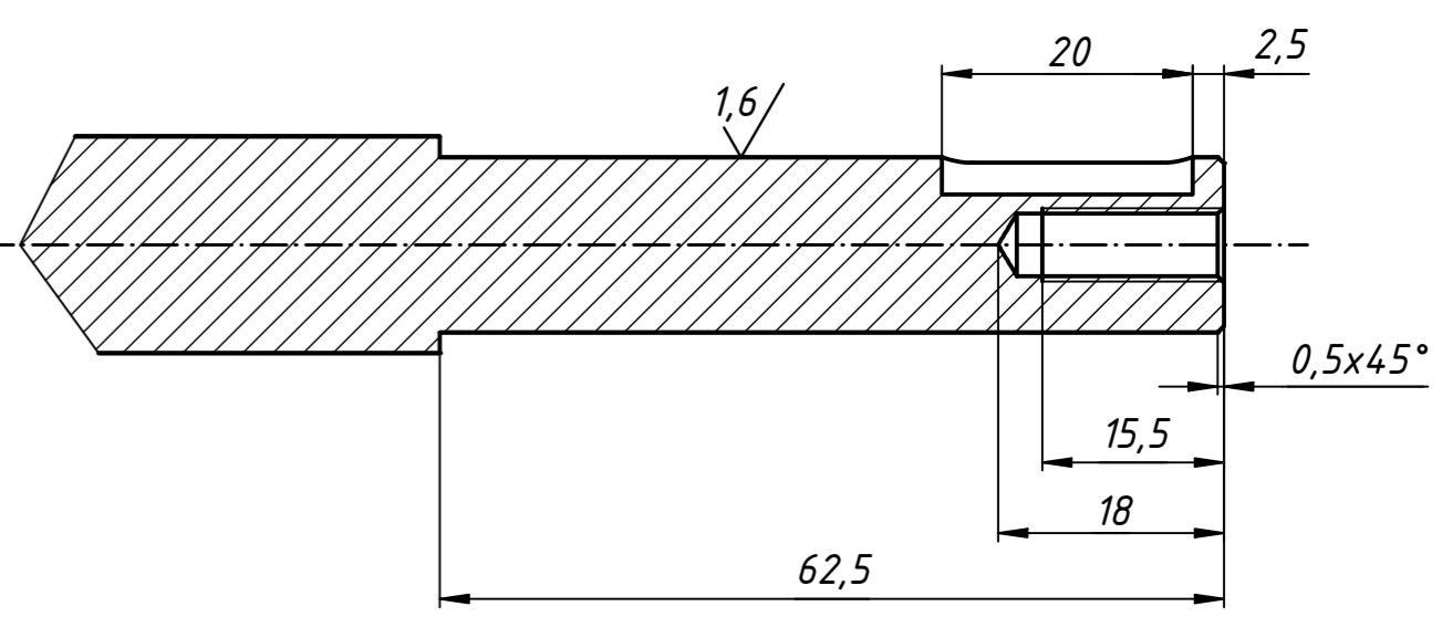
C-C (1.5:1)
