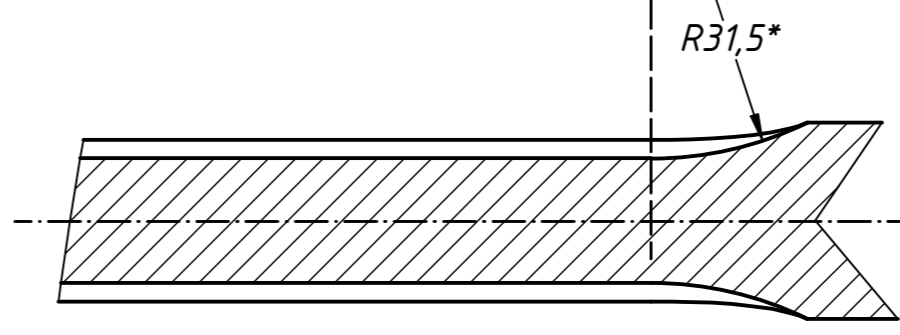
G-G (1.5:1)
